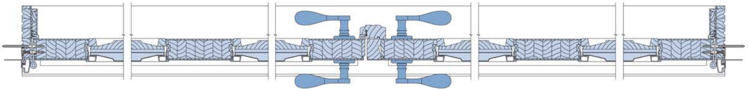
Double Door Frame Horizontal Section - 2 Panel
