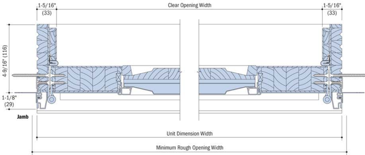
Double Door Frame Horizontal Section - 1 Panel
