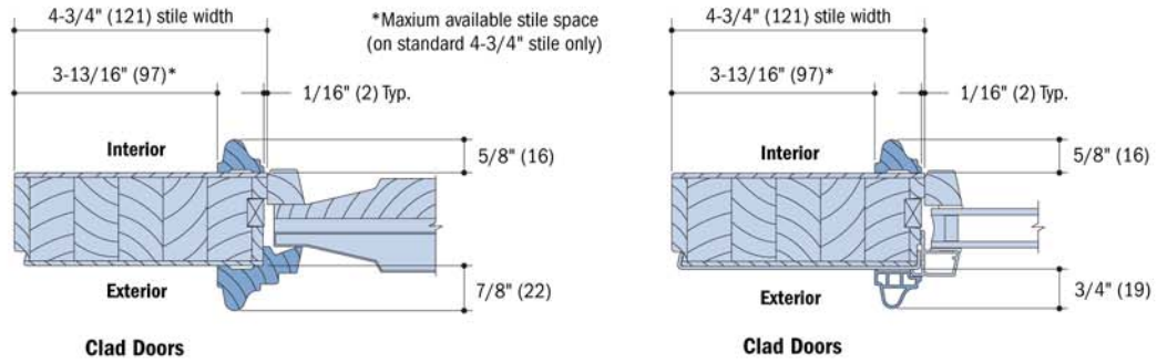
Typical Raised Molding Options (panels and transoms)
