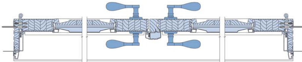
Double Door Frame Horizontal Section through the panel
