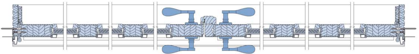
Horizontal Section - 3 Panel
