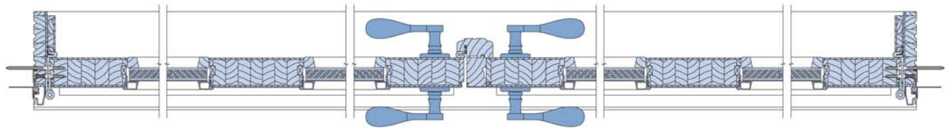
Horizontal Section - 2 Panel
