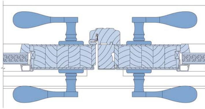
Double Door Frame Single Panel
