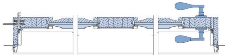
Single Door Frame Horizontal Section - 2 Panel
