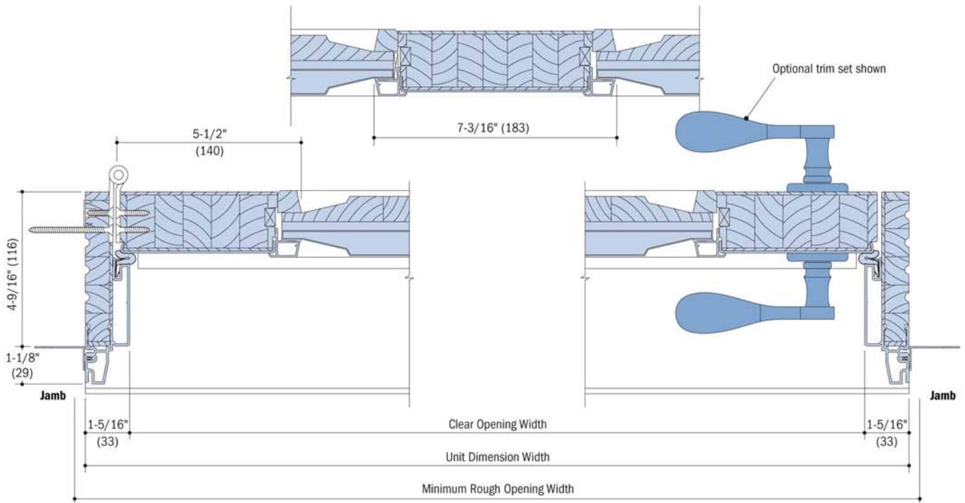
Single Door Frame Horizontal Section - 2 Panel
