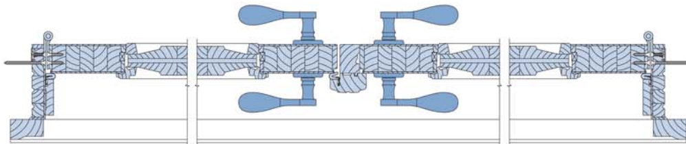
Horizontal Section - through the panel
