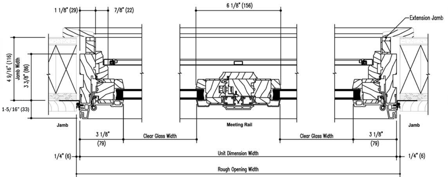
Horizontal Section
