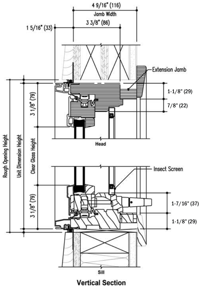
Vertical Section
