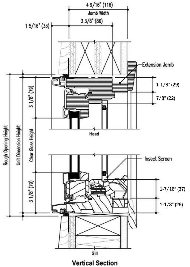
Vertical Section
