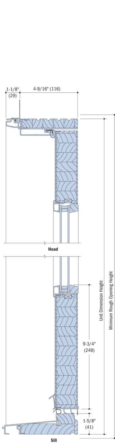
Vertical Section - Full Lite
