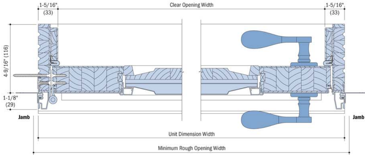
Single Door Frame Horizontal Section - 1 Panel
