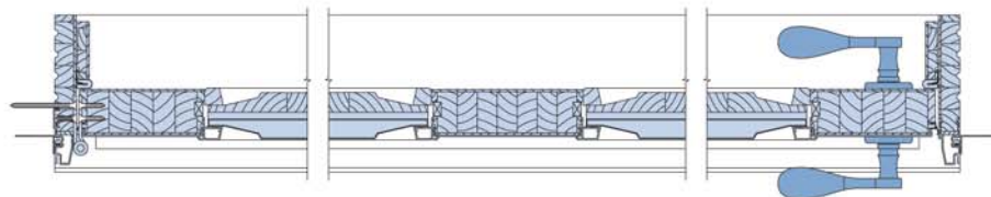
Single Door Frame Horizontal Section - 2 Panel
