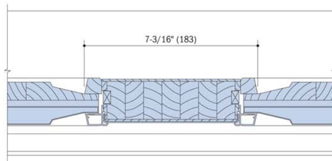
Single Door Frame Horizontal Section - 2 Panel
