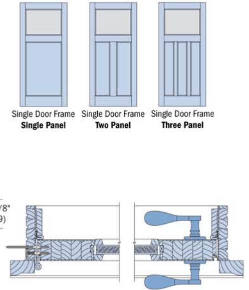
Horizontal Section - 1 Panel
