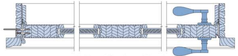
Horizontal Section - 2 Panel
