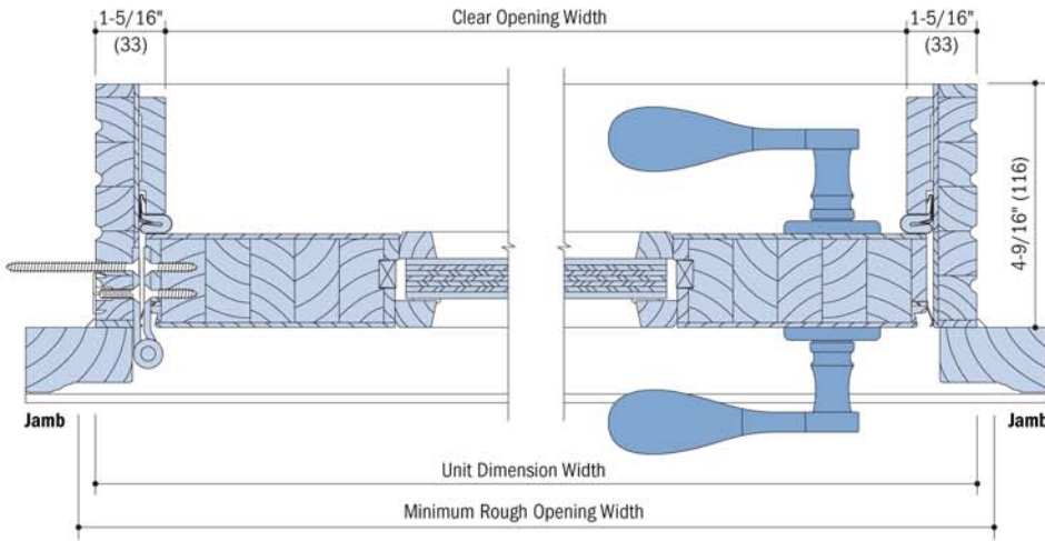
Horizontal Section - 1 Panel
