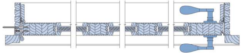
Horizontal Section - 3 Panel
