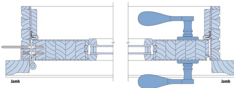
Horizontal Section - through the glass
