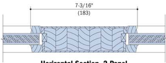
Horizontal Section - 2 Panel
