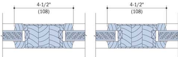
Horizontal Section - 3 Panel
