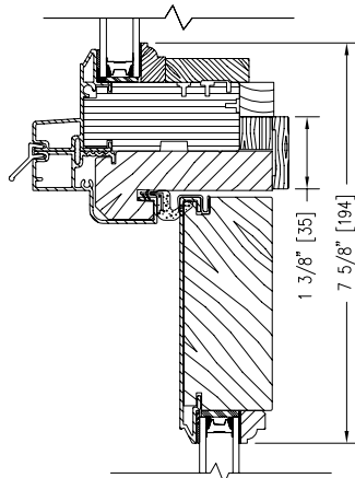
AUXILIARY OVER INSWING DOOR
