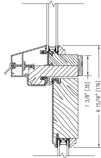
DIRECT GLAZED TRANSOM OVER INSWING DOOR
