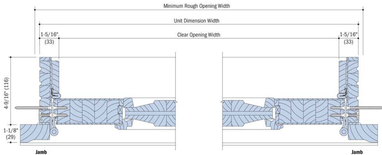
Double Door Frame Horizontal Section - 1 Panel
