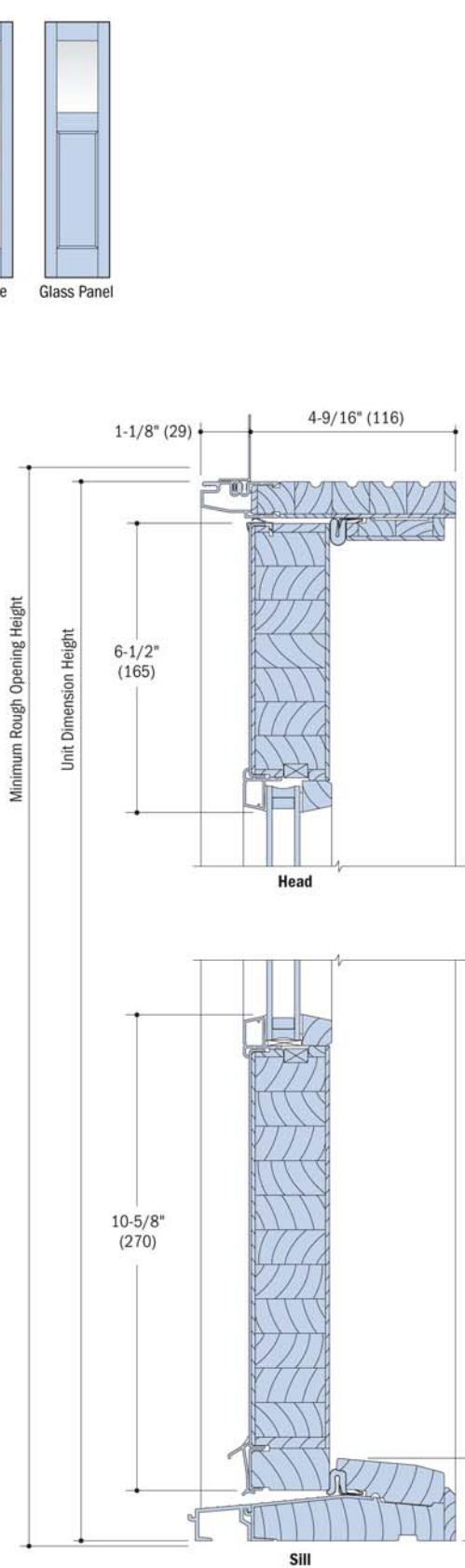
Vertical Section Full Lite
