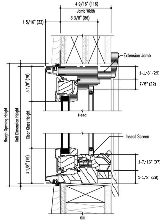
Vertical Section
