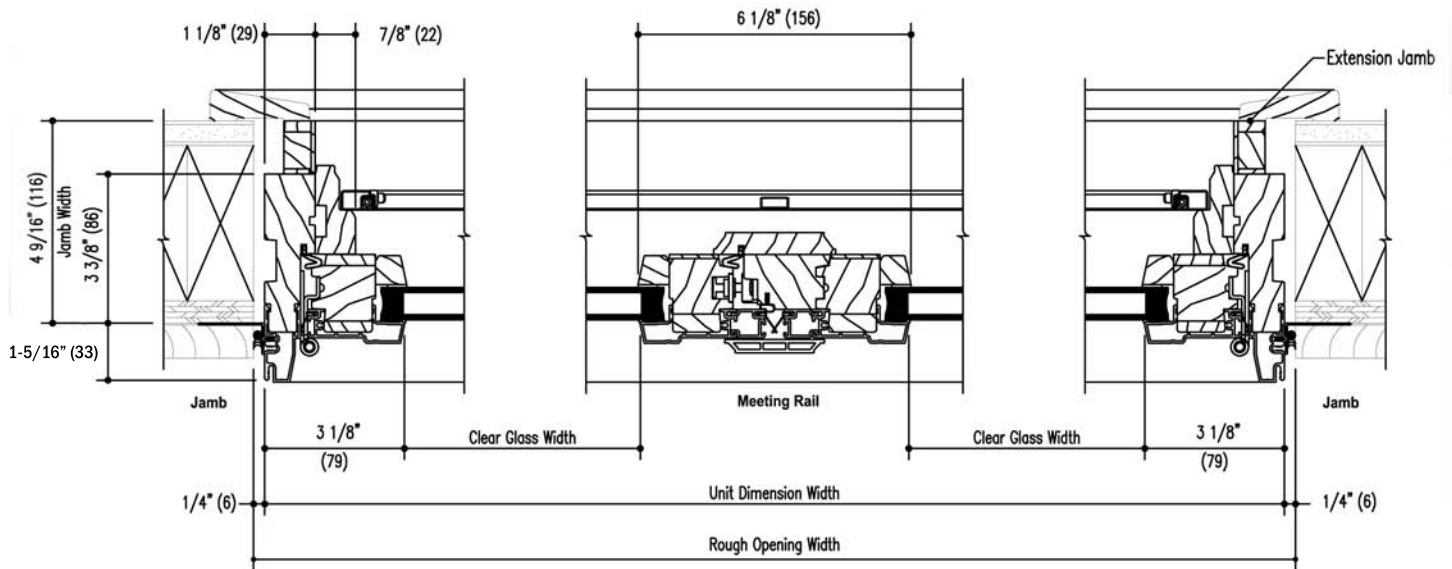
Horizontal Section
