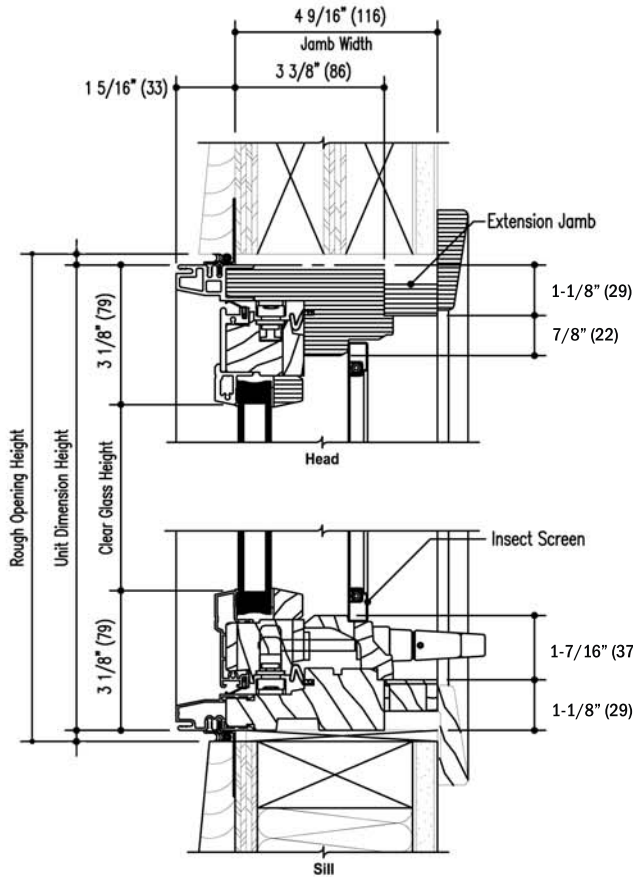
Vertical Section
