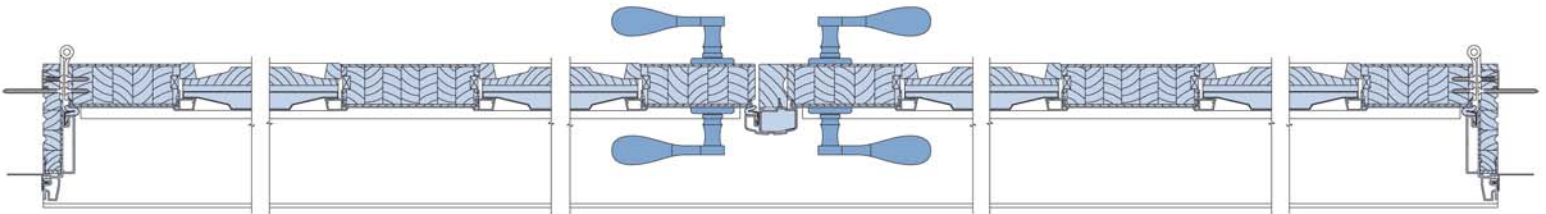
Double Door Frame Horizontal Section - 2 Panel
