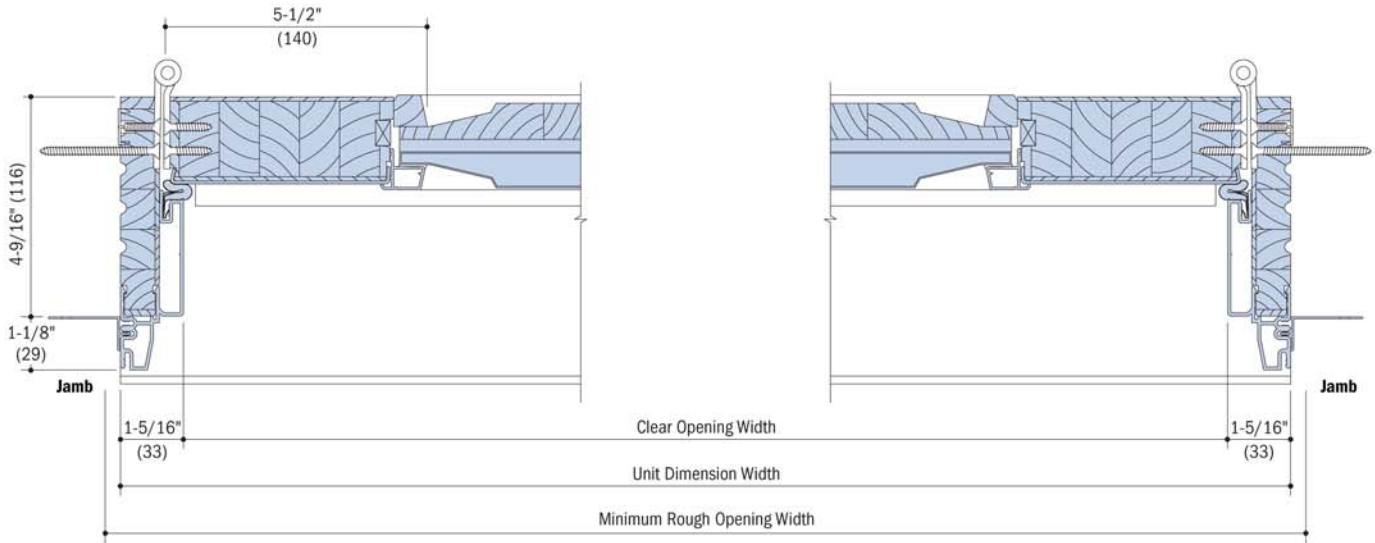
Double Door Frame Horizontal Section - 2 Panel
