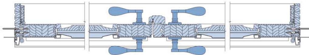
Double Door Frame Horizontal Section - through the panel
