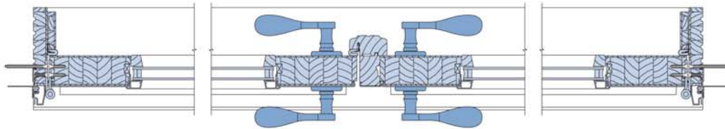
Double Door Frame Horizontal Section - through the glass
