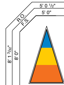
TRIANGLE
