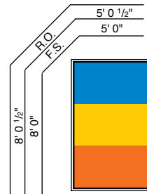
RECTANGLE
