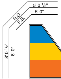
PENTAGON
