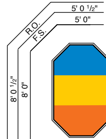
OCTAGON
