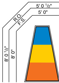
TRAPEZOID
