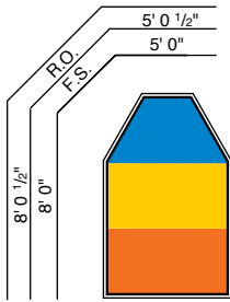
HEXAGON
