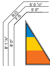
RIGHT TRIANGLE
