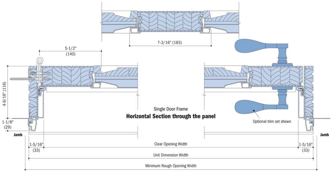
Horizontal Section through the panel
