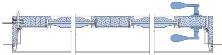
Single Door Frame
