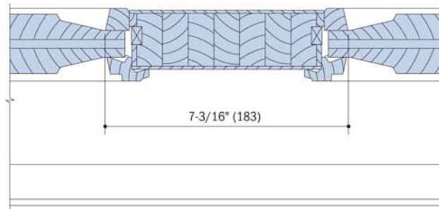
Horizontal Section - 2 Panel
