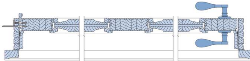
Horizontal Section - 2 Panel
