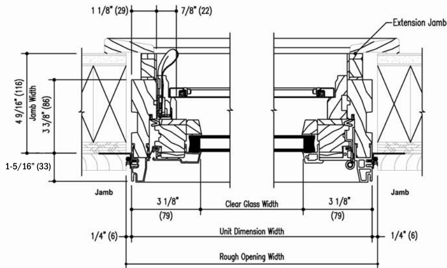
Horizontal Section
