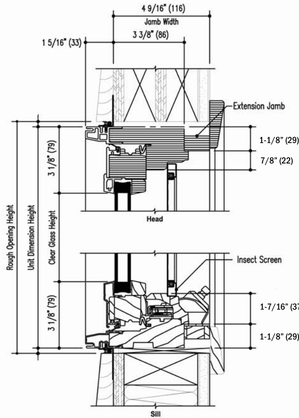
Vertical Section
