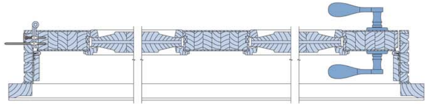
Horizontal Section - through the panel
