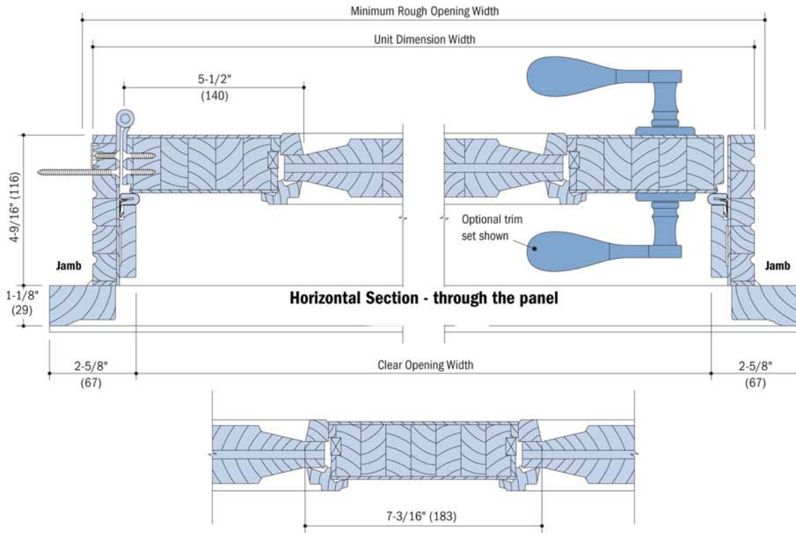
Horizontal Section - through the panel
