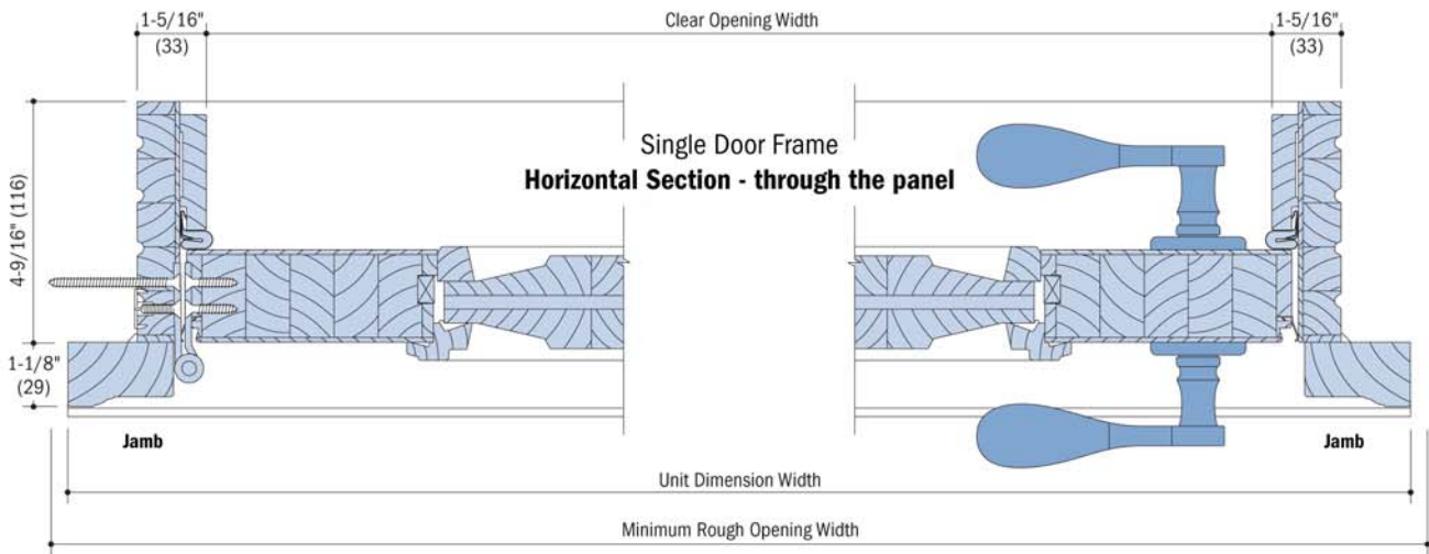
Single Door Frame Horizontal Section - through the panel
