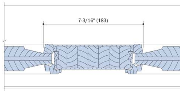
Horizontal Section - 2 Panel
