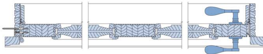
Horizontal Section - 2 Panel
