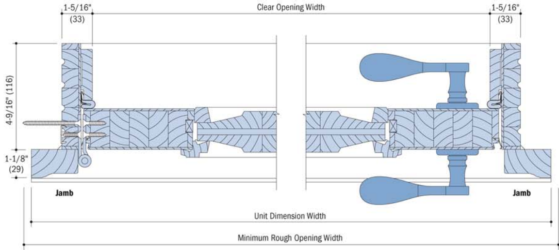
Horizontal Section - 1 Panel
